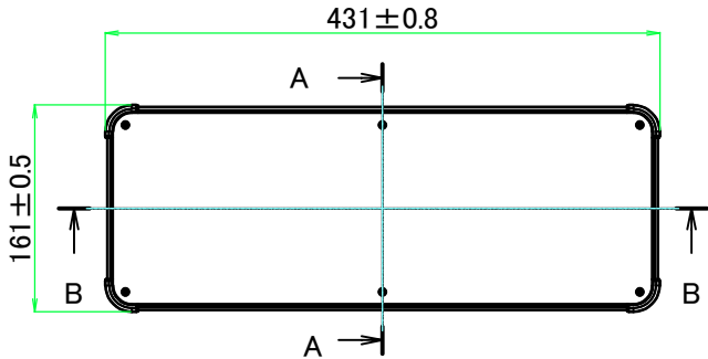
E view
